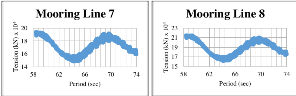
Figure 9. Tension of mooring line using SLFR
