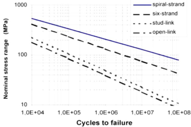
Figure 5. S-N Curve
