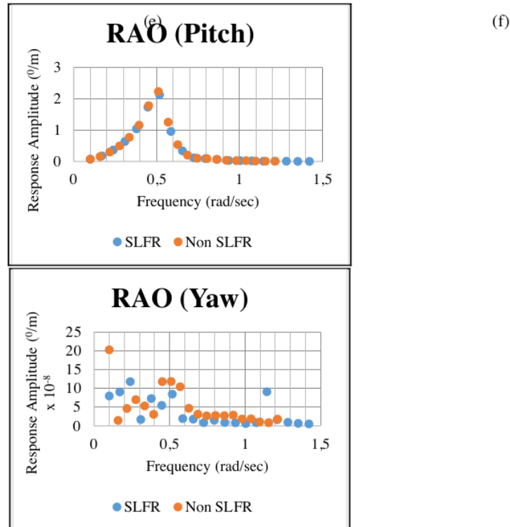
9 Figure 8. Comparison of RAO using SLFR and without SLFR; (a) surge motion, (b) sway motion, (c) heave motion, (d) roll motion, (e) pitch motion and (f) yaw motion
