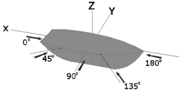
Figure 3. Heading direction in Ansys software
