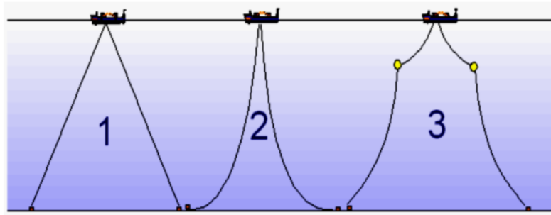
Figure 4. Mooring System Configurations; (1) taut Mooring, (2) catenary Mooring, and (3) catenary mooring with buoyancy
