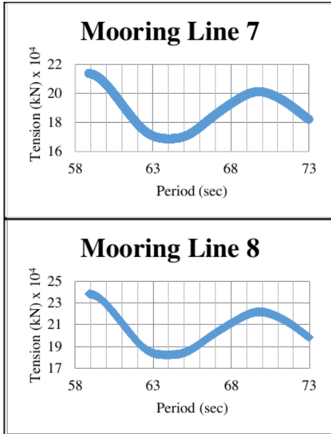
Figure 10. Tension of mooring line without using SLFR
